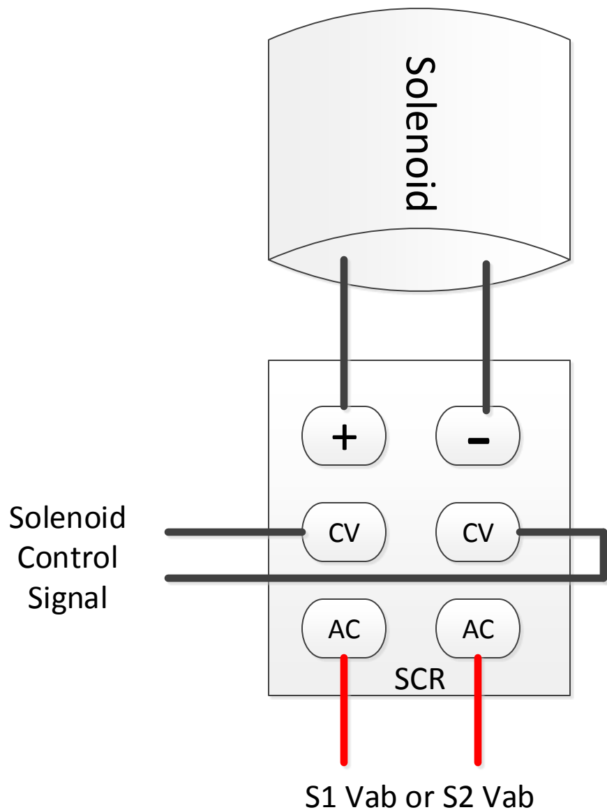
Fig 1: Before Modification
