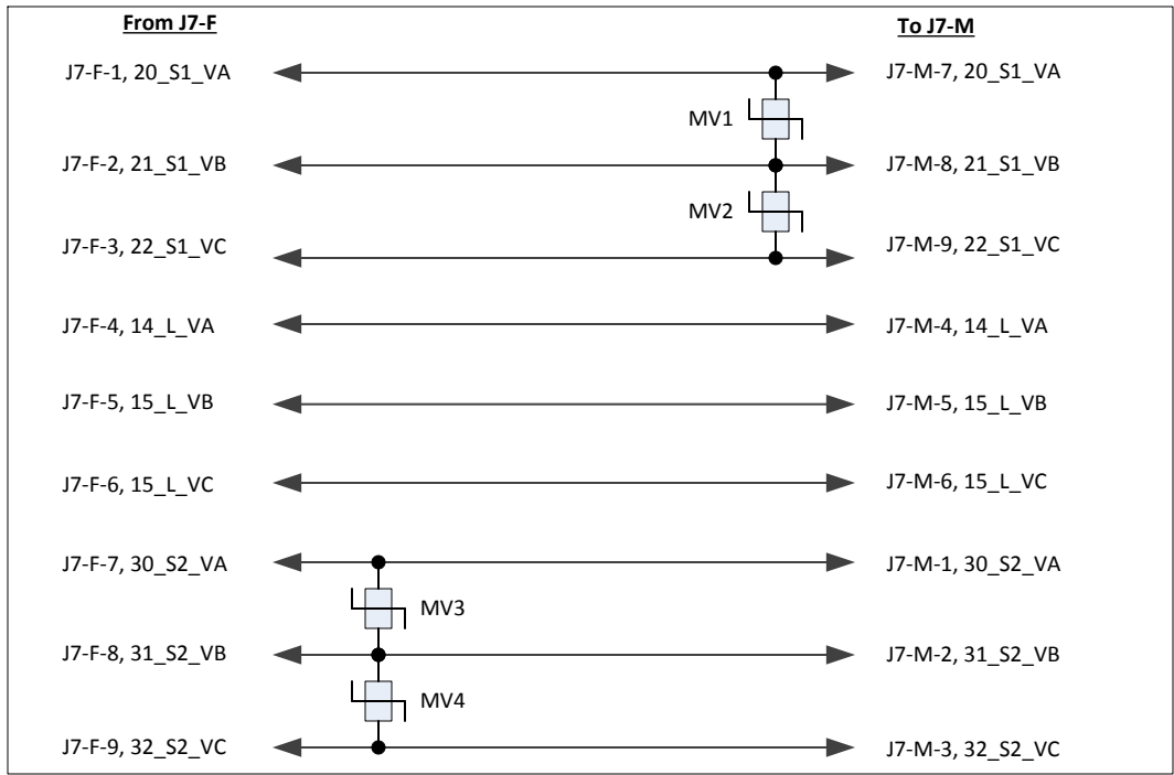
Fig 3: MX150/250 J7 Conversion Harness for line voltages
