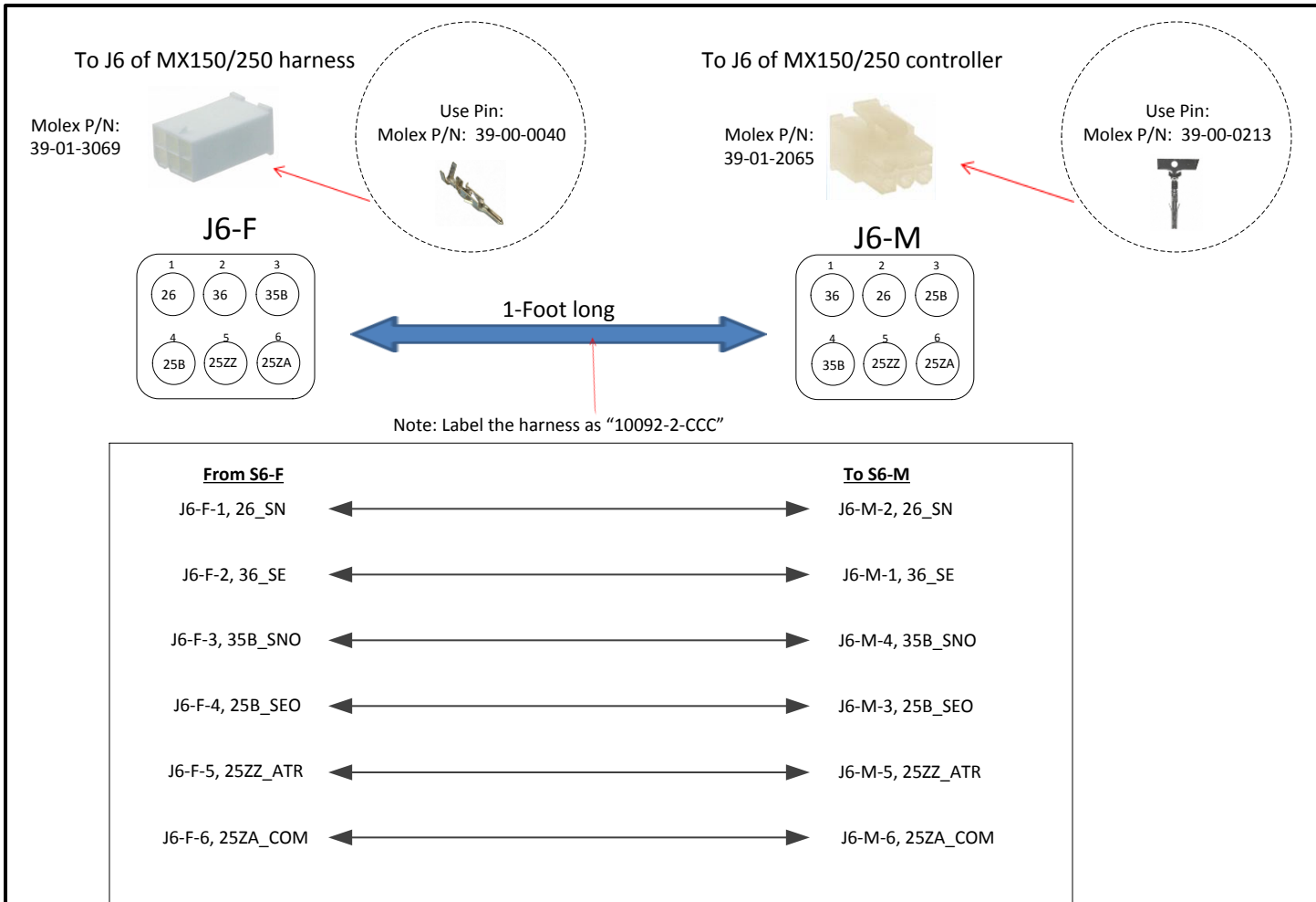
Fig 2: MX150/250 J6 Conversion Harness for Limit Switch Signals
